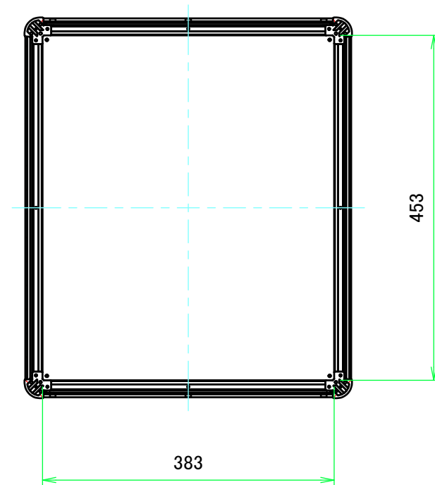
B-B (1:7)
