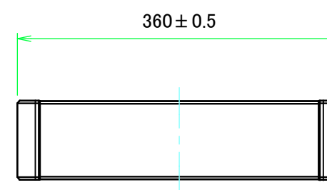
C view
