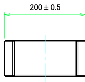
C view
