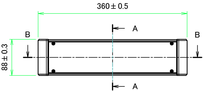
A view
