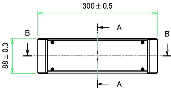
A view
