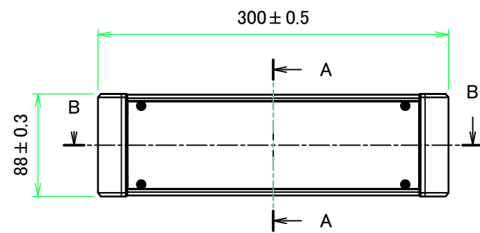
A view
