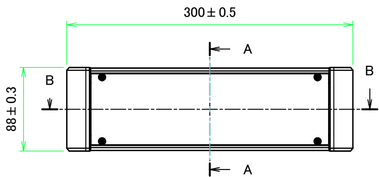
A view
