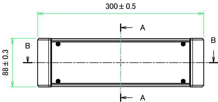
A view
