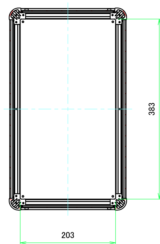
B-B (1:5)
