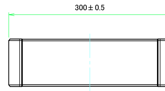
C view
