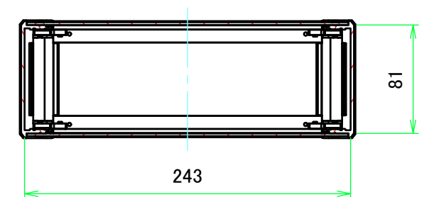
C-C (1:4)
