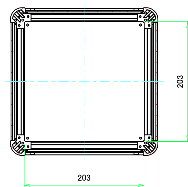
B-B (1:4)
