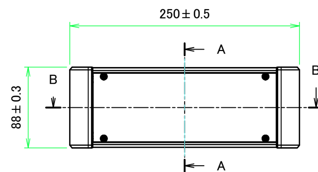
F view
