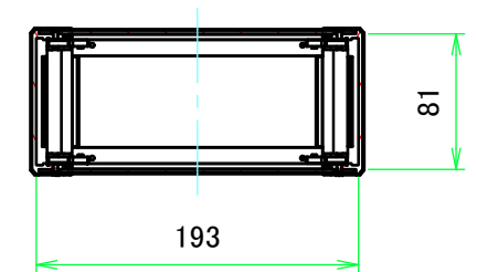
C-C (1:5)
