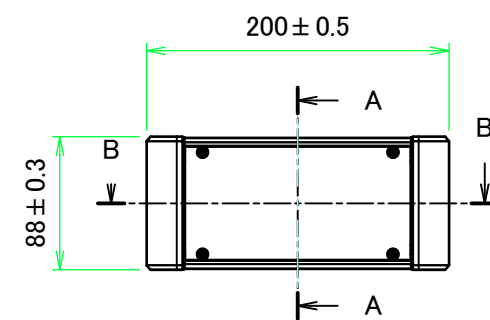
A view
