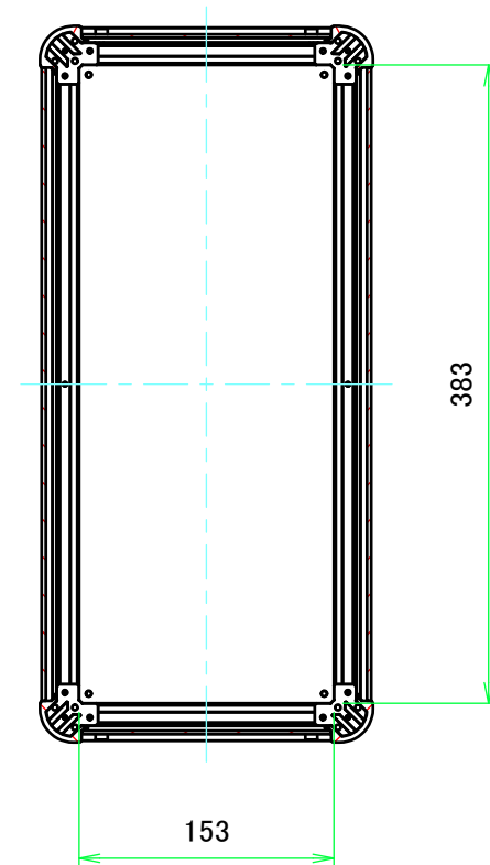
B-B (1:5)
