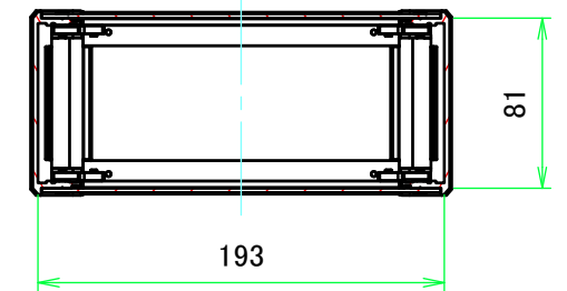
C-C (1:4)
