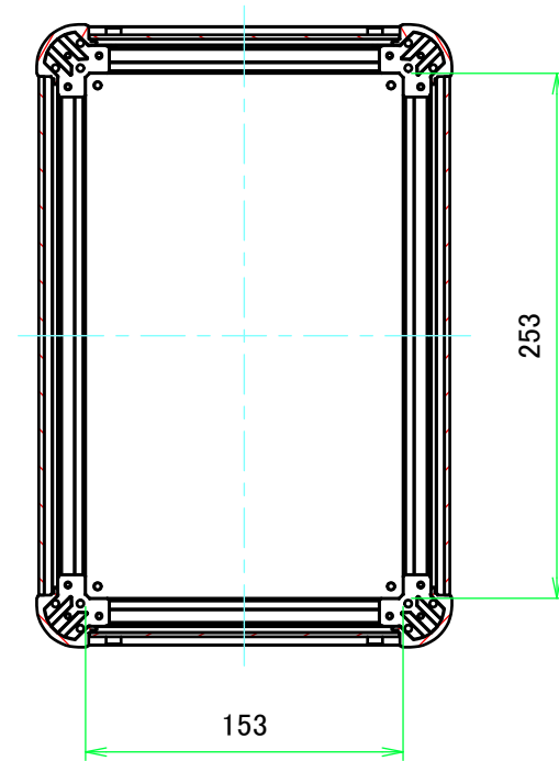
B-B (1:4)
