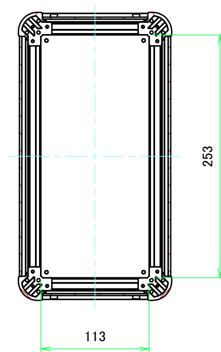
B-B (1:4)
