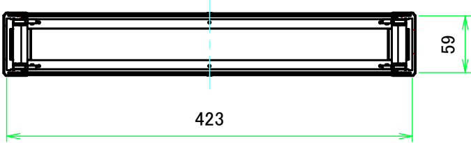
C-C ( 1:5.5 )
