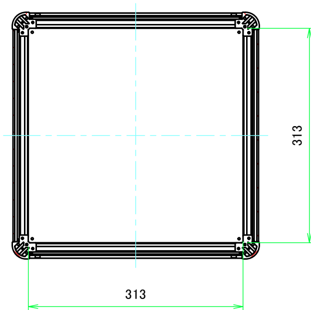
B-B ( 1:5.5 )
