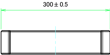
C view
