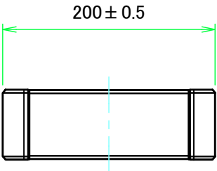
C view
