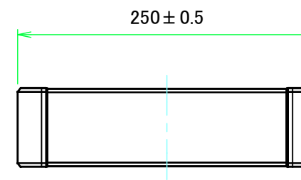
C view
