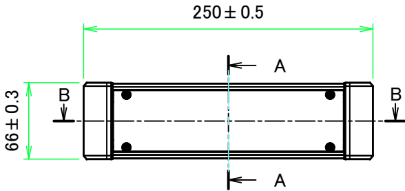
A view
