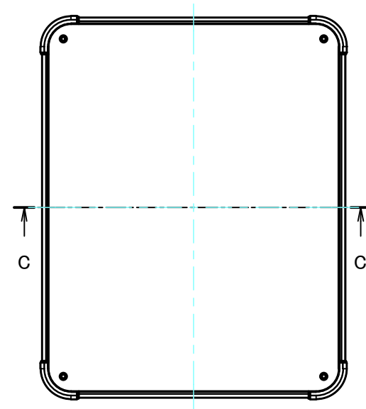
E view
