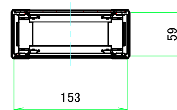
C-C (1:5)
