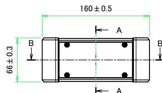
A view
