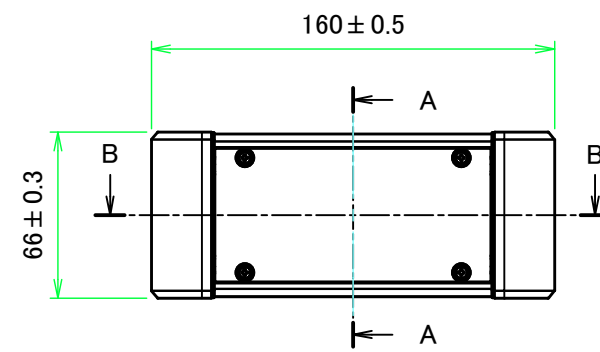
A view
