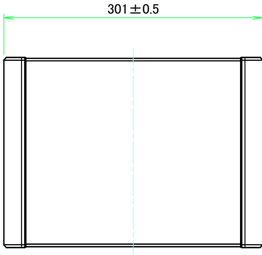
C view
