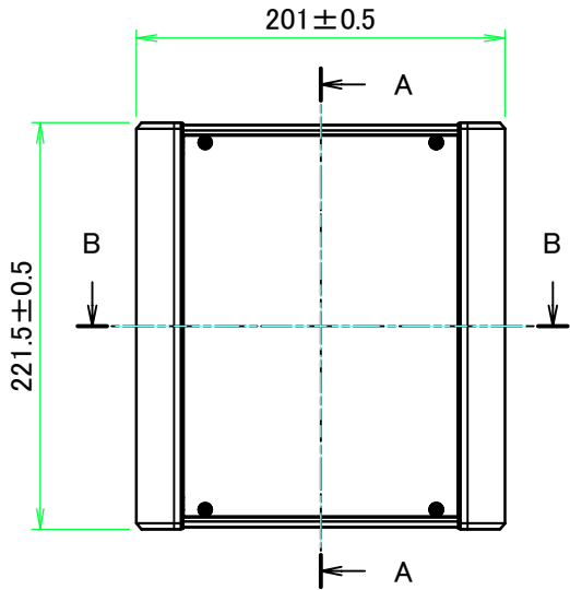
A view
