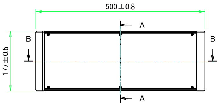
A view
