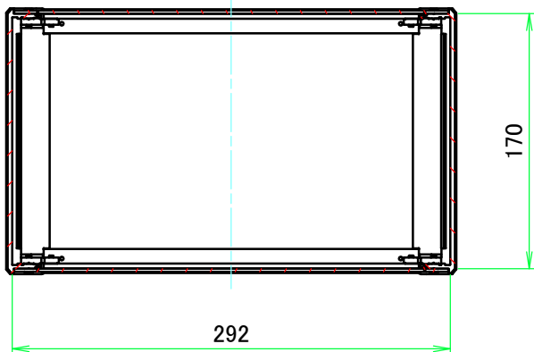
C-C ( 1 :4.5 )
