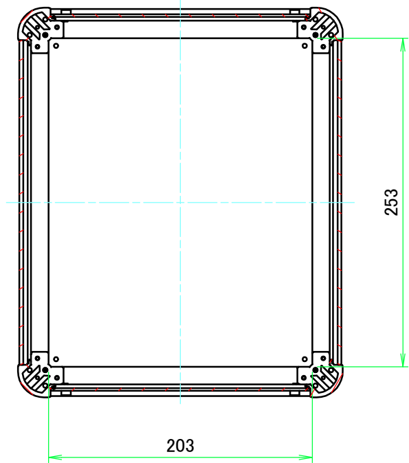
D view
