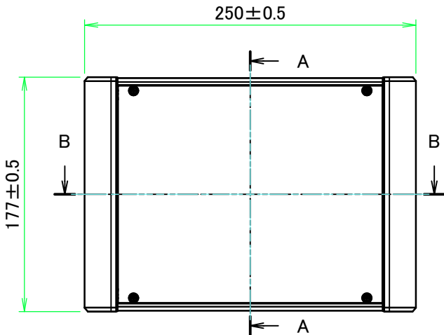
A view
