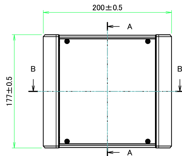
F view
