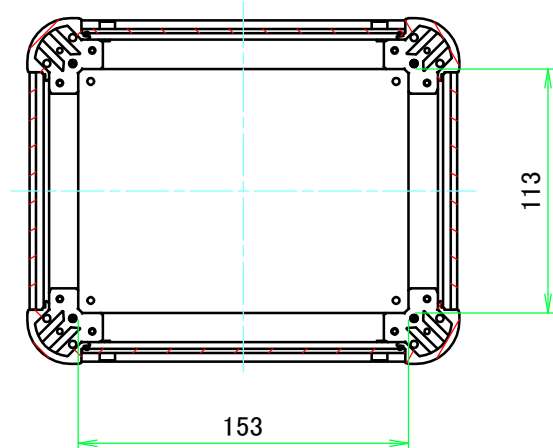
B-B ( 1 :3.5 )
