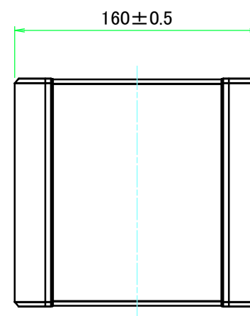
C view
