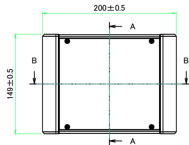
A view
