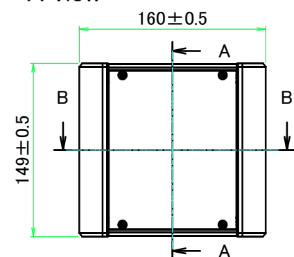
A view
