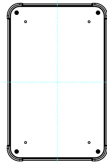
F view
