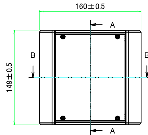
A view
