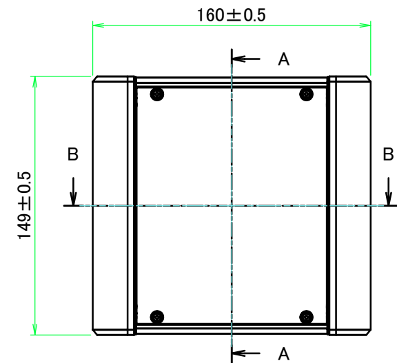
A view
