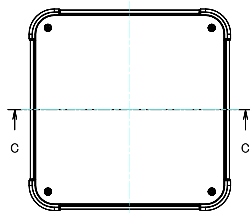
E view
