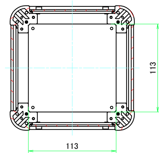
B-B (1:3)
