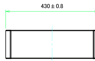
C view
