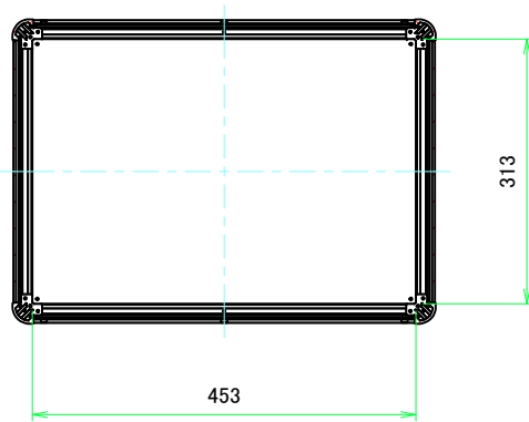
B-B (1:7)
