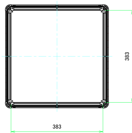
B-B (1:6.5)
