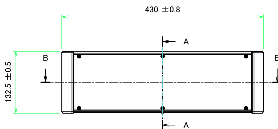
F view
