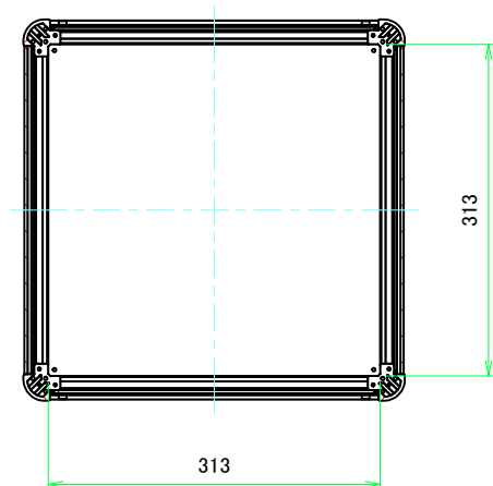
B-B (1:5.5)
