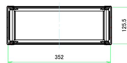
C-C (1:5.5)
