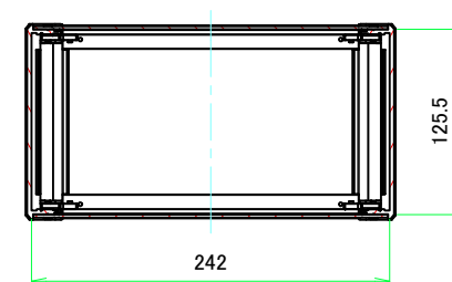
C-C (1:4)
