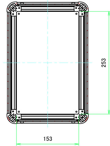
B-B (1:4)
