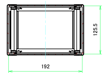
C-C (1:4)
