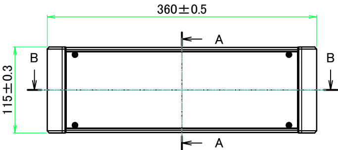
A view
