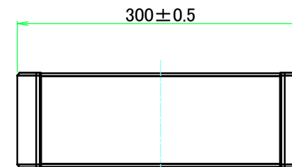
C view
