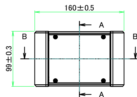
A view
