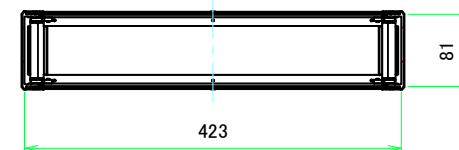
C-C (1:6)
