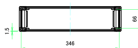
A-A (1:5.5)
