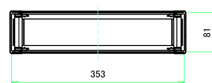
C-C (1:5.5)
