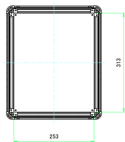
B-B (1:5)
